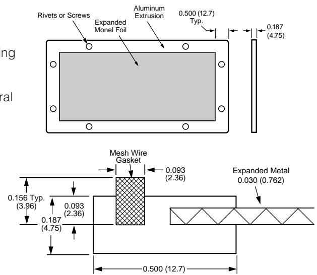
Frame Design 61-448
