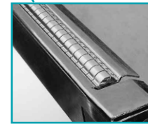
Be-Cu fingerstock,
