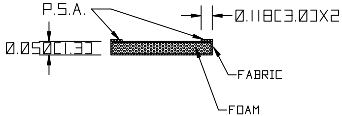
SECTION A-A ENLARGED
