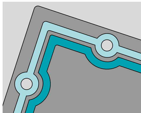
Molding a non-conductive elastomer to the outboard edge and around bolt holes further protects the inboard conductive elastomer and the enclosure in corrosive environments.
