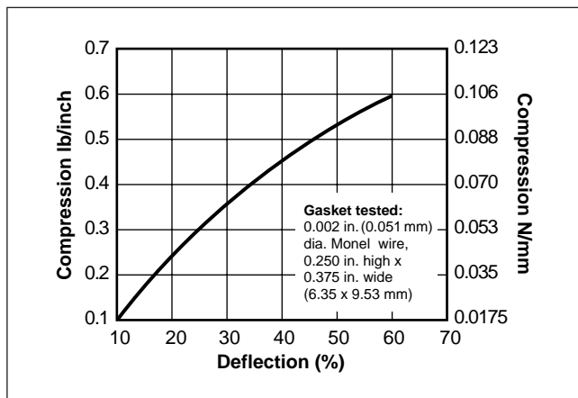
Figure 1 Compression-Deflection
